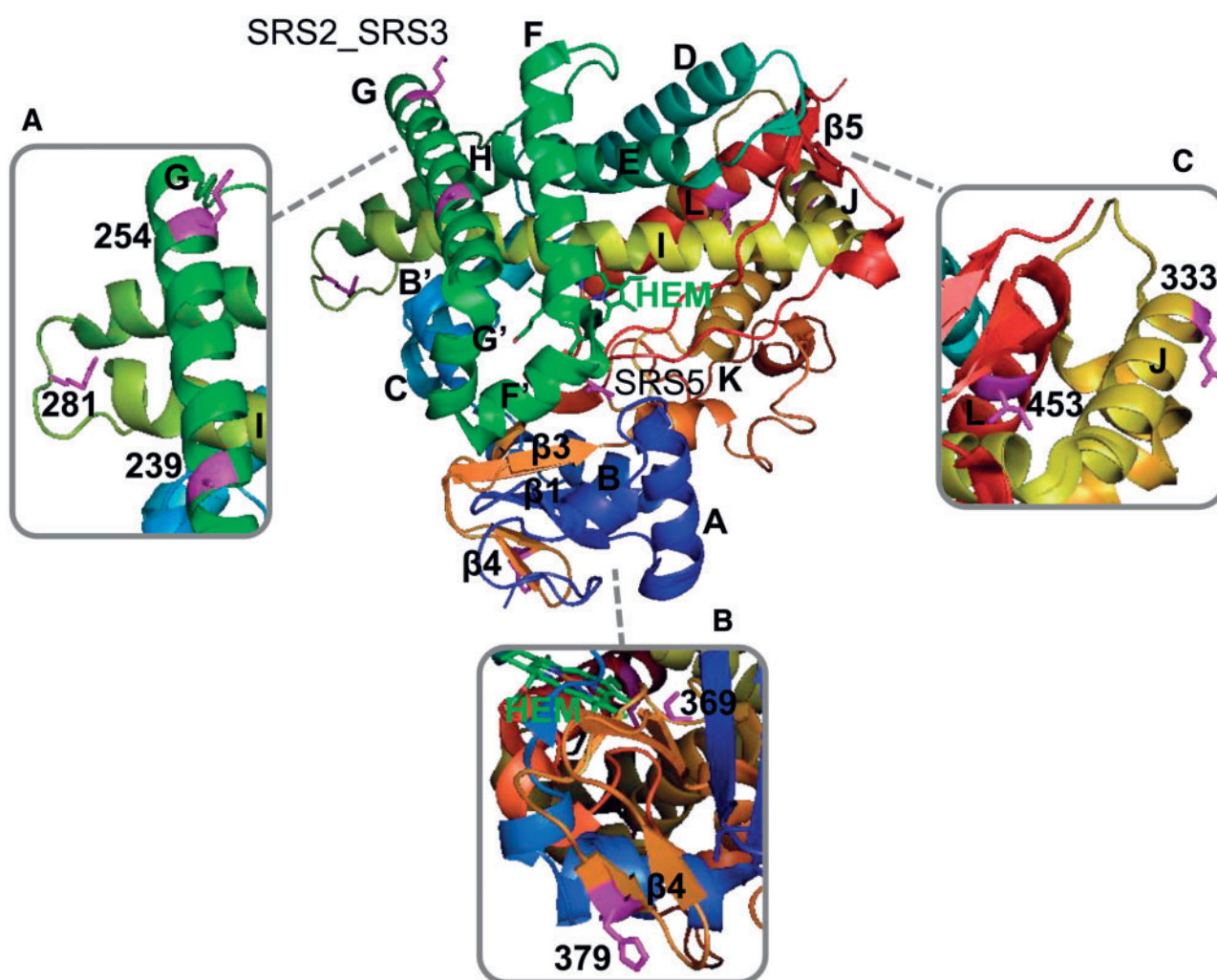
FIG. 5. —3D analyses of sites detected to be under positive selection in the avian CYP2C. The CYP2C 3D structure predicted in this study is superimposed to its CYP2C8 template (2VN0 human). The positively selected sites are shown as pink sticks, indicating the corresponding amino acid. The regions corresponding to the helices are named with the corresponding capital letter and the \beta -structures are named with a \beta followed by a number. HEM represents the heme group. Two SRS regions are represented: SRS2_SRS3 (top) and SRS5 (bottom).
