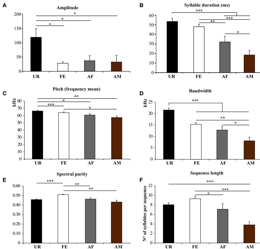
FIGURE 5 | Characteristics of syllables and sequence length in different contexts. (A) Amplitude. *p < 0.025 after Benjamini and Hochberg correction. (B) Syllable Duration (milliseconds) *p < 0.041 , **p < 0.005 , ***p < 0.0001 after correction. (C) Frequency mean. *p < 0.033 , **p < 0.005 , ***p < 0.0001 after correction. (D) Frequency range or Bandwidth. *p < 0.041 , **p < 0.005 , ***p < 0.0001 after
