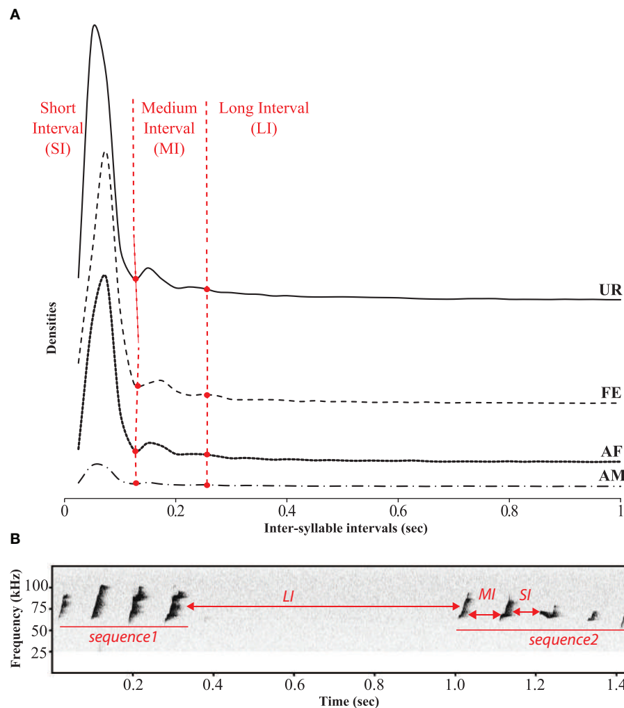
FIGURE 7 | Temporal organization of sequences in different context. (A) Distribution of the inter-syllables intervals for the four conditions defining three types of silent intervals between sequences of syllables. (B) Representation of these three types of intervals on a sonogram separating two songs by a long interval.
