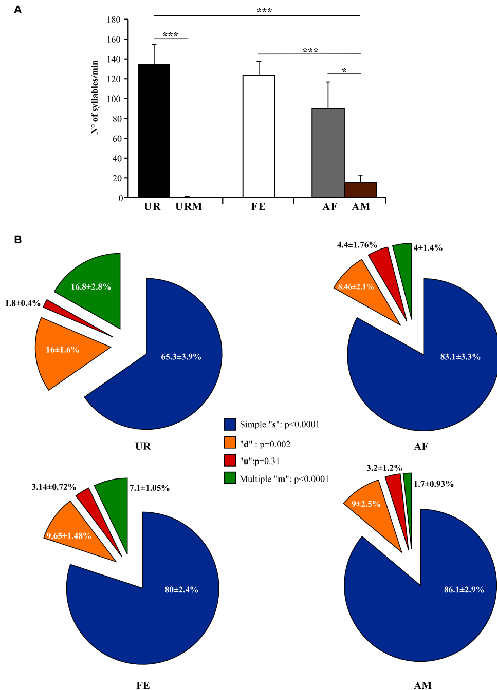
FIGURE 3 | Number of syllables emitted and repertoire across conditions. (A) Call rate (number of USVs per minute). Data are presented as mean ± SEM ( n = 12 males). * p < 0.03 , *** p < 0.0001 for post-hoc Student's paired t -test after Benjamini and Hochberg
