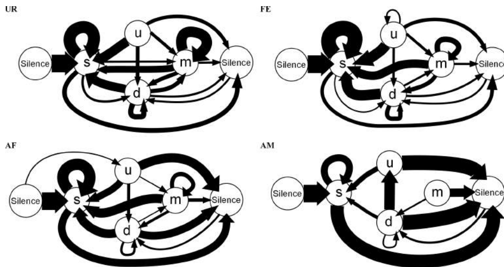
FIGURE 10 | Graphical representation of sequences of conditional syllable transition probabilities for each context. Diagrams represent the conditional probability of occurrence (for the probabilities above the threshold of p = 0.05 ) of a transition type in each context averaged from n = 12 males. Thickness is proportional to the P
